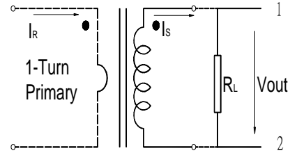
Test Circuit
